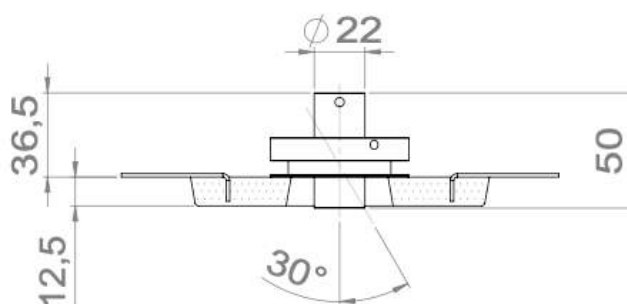
CROSS-SECTION A-A SCALE 1 : 2
