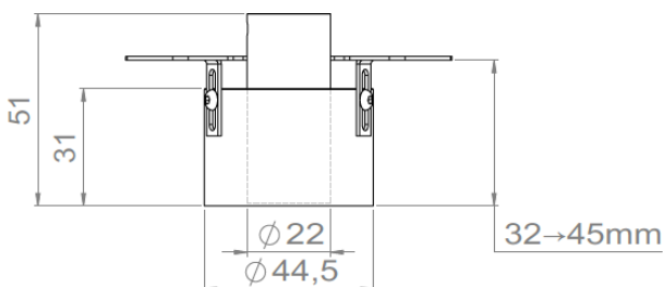
Upside down fixing brackets version
