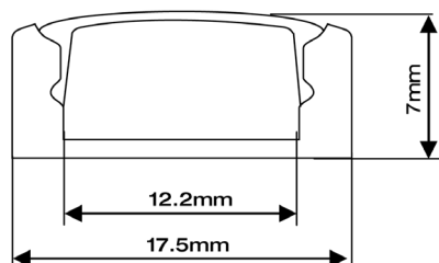
Natural anodized aluminum profile
