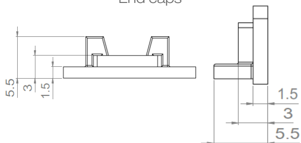
End caps
