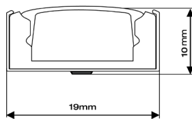
Fixing clip
