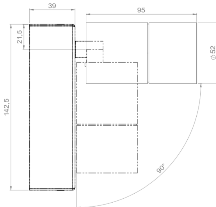
AUORE D52 Rectangular Wall-mounted – Length 95mm ≤ 13W
