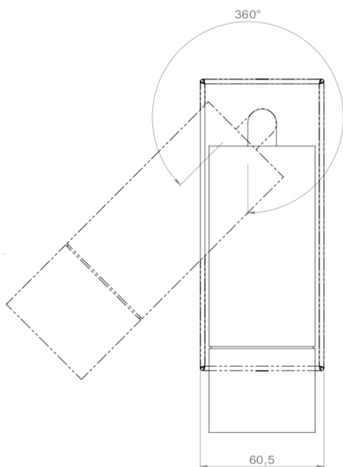
AUORE D52 Rectangular Wall-mounted – Length 140mm ≤ 13W
