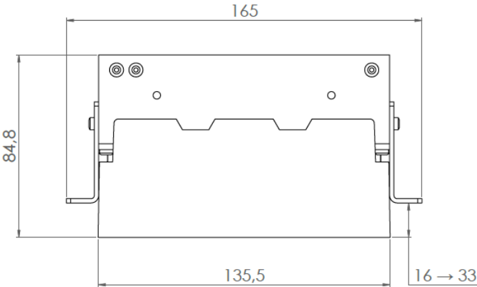
Version IP20
