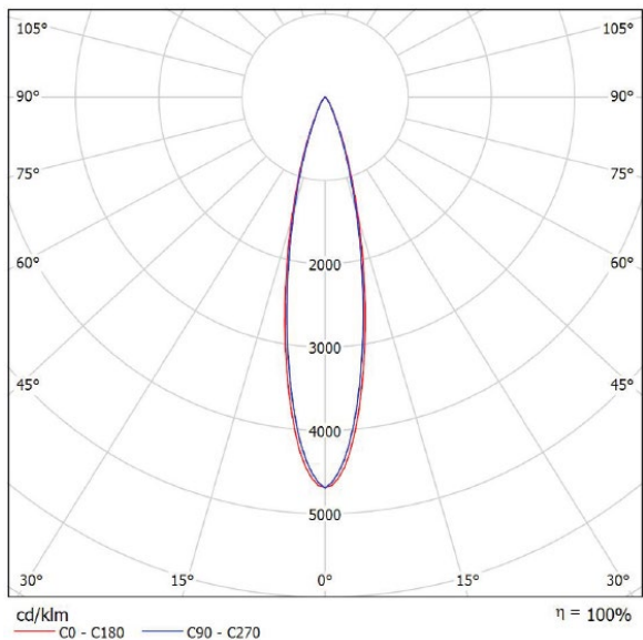
21° version
