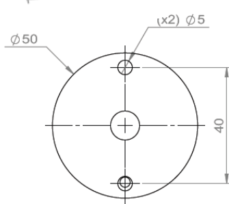
On-plate version
