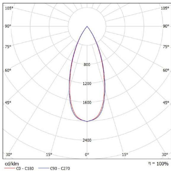
44° version
