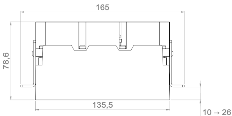
IP54 version
